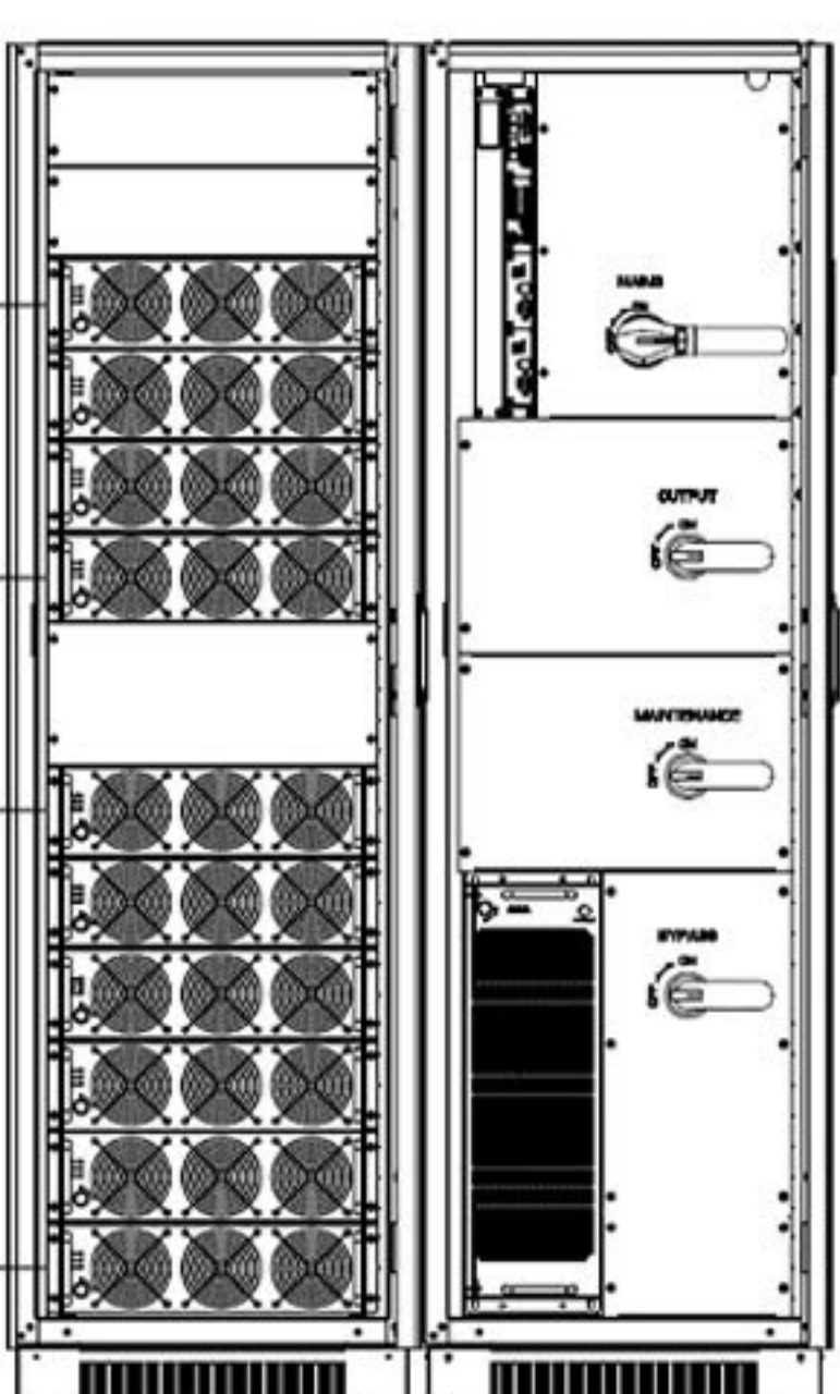
Front View: Full configuration (door open)
